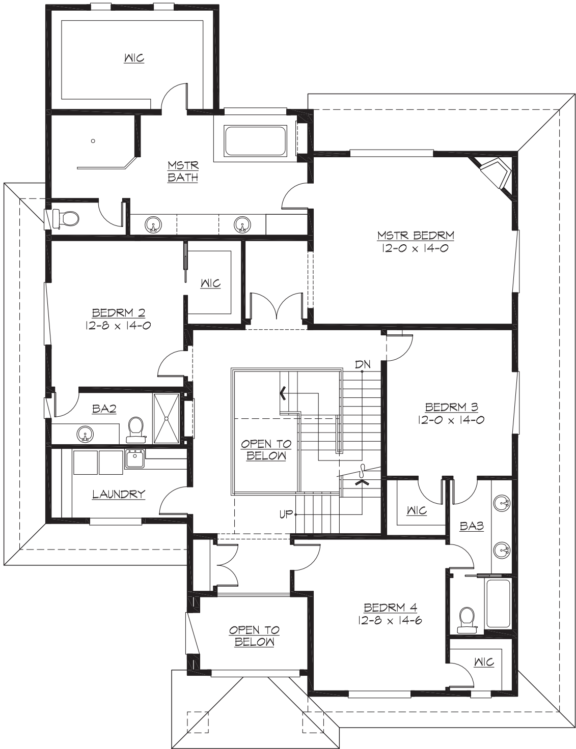
UPPER FLOOR
